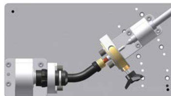
Checking jig PV 100 F with standard torch head and optionally Aligning module
