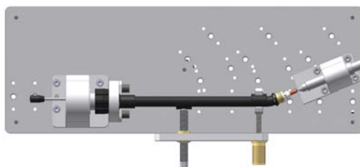
Checking jig PV 150 XL with torch head XL version, optionally straightening set PVR 102, Aligning bracket JH 100 and support set PVS 102 with torch adapter PVP 102
