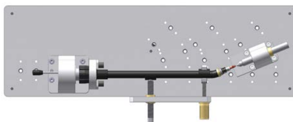
Checking jig PV 160 XL with torch head XL version, optionally straightening set PVR 102, Aligning bracket JH 100 and support set PVS 102 with torch adapter PVP 102
