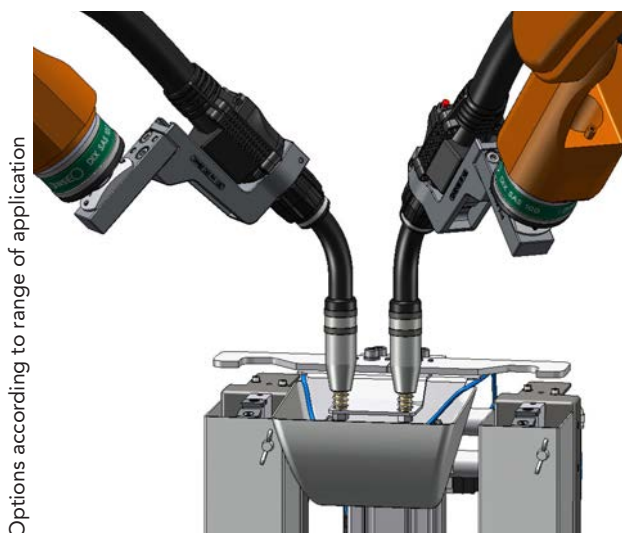
Application sample: Cleaning process of the gas nozzle
