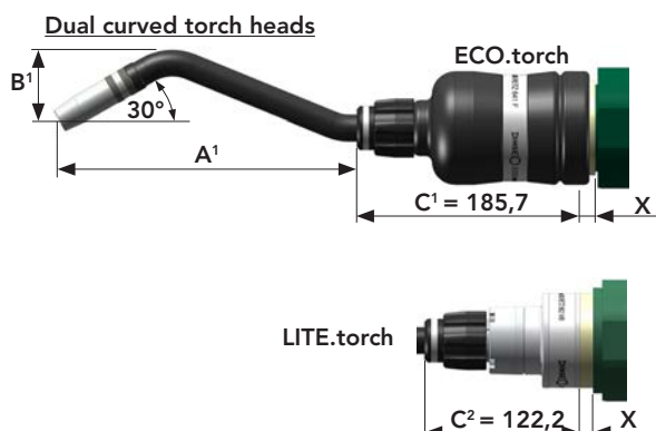
TCP dimensions for torch heads at hollow wrist robotic application with rotary interface ECO.torch, LITE.torch, T.Connector HW(D) or Frontdrive-Connector
