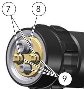
MFTZ torch head
