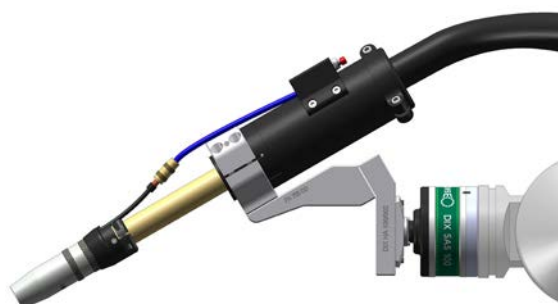
Torch bracket, fixed PHF 730 DD with shock sensor DIX SAS 100/002 (sample application)
