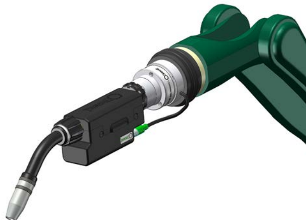
Hollow wrist robot with torch head, drive unit and T.Connector HWD, application sample
