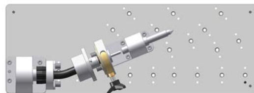
Checking jig PV 100 XL with standard torch head and optionally Aligning module
