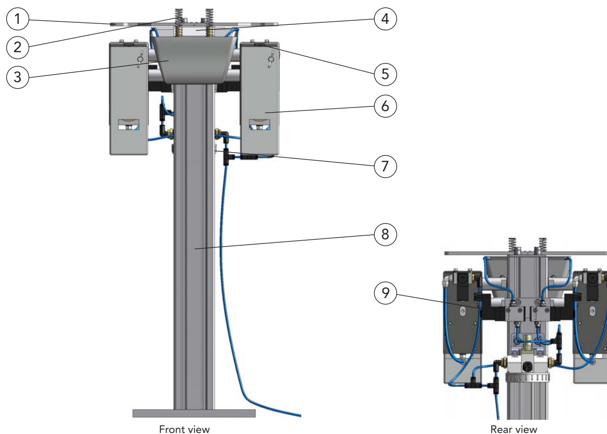
Torch cleaning station DIX PRS 1000 D
