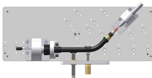
Checking jig PV 100 XL with torch head XL version, optionally straightening set PVR 102, aligning bracket JH 100 and support set PVS 102 with torch adapter PVP 102
