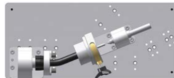
Checking jig PV 158/003 with standard torch head and optionally Aligning module
