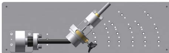
Checking jig PV 160 XL with standard torch head and optionally Aligning module
