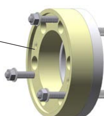
Application sample with additional adapter
