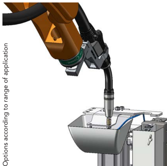
Application sample: Cleaning process of the gas nozzle
