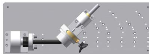
Checking jig PV 150 XL with standard torch head and optionally Aligning module
