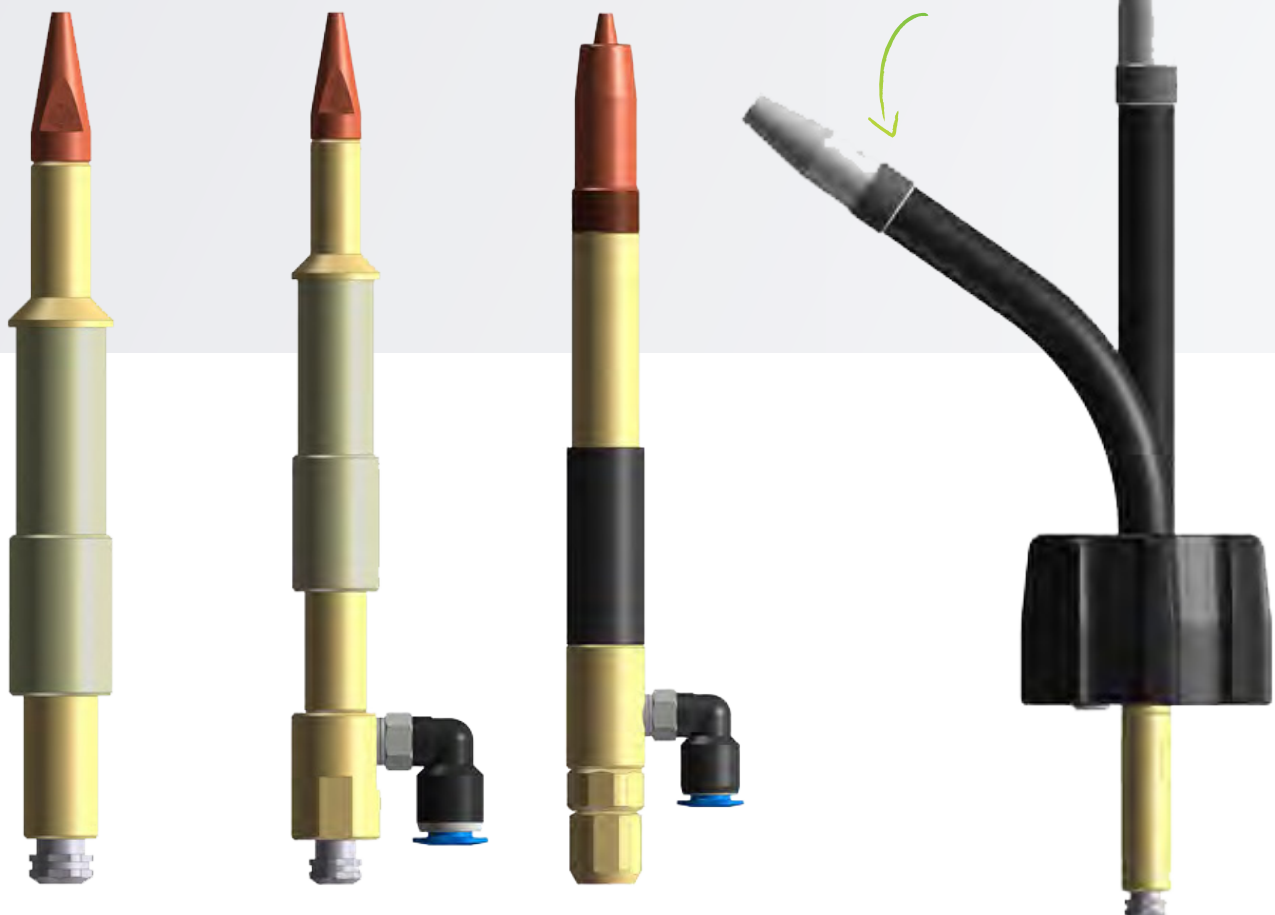
DIX LH 100 AW Gas cooled, without integrated shield gas guidance
